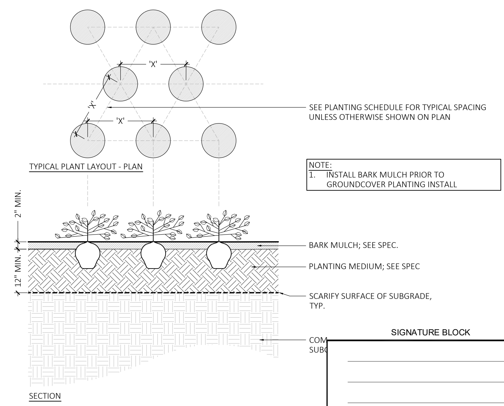
2 GROUNDCOVER PLANTING SCALE: 3/4" = 1'-0"
