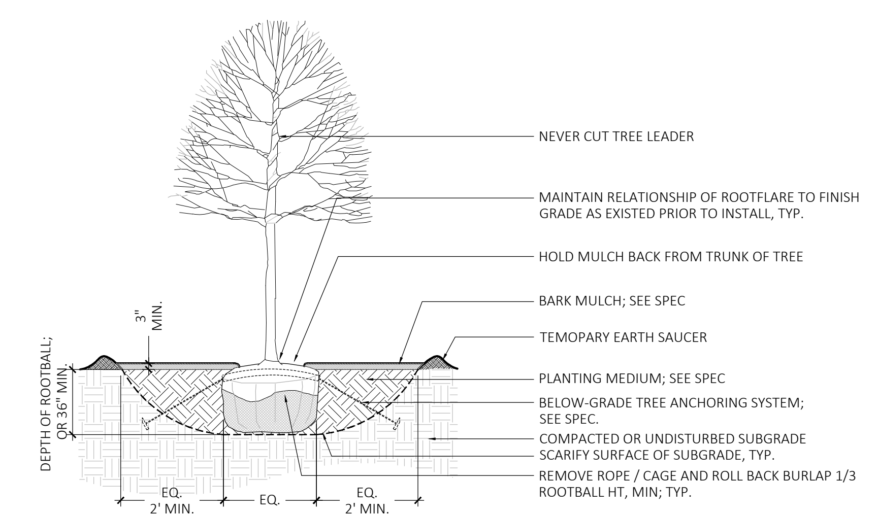
4 DECIDUOUS TREE PLANTING SCALE: 3/8" = 1'-0"
