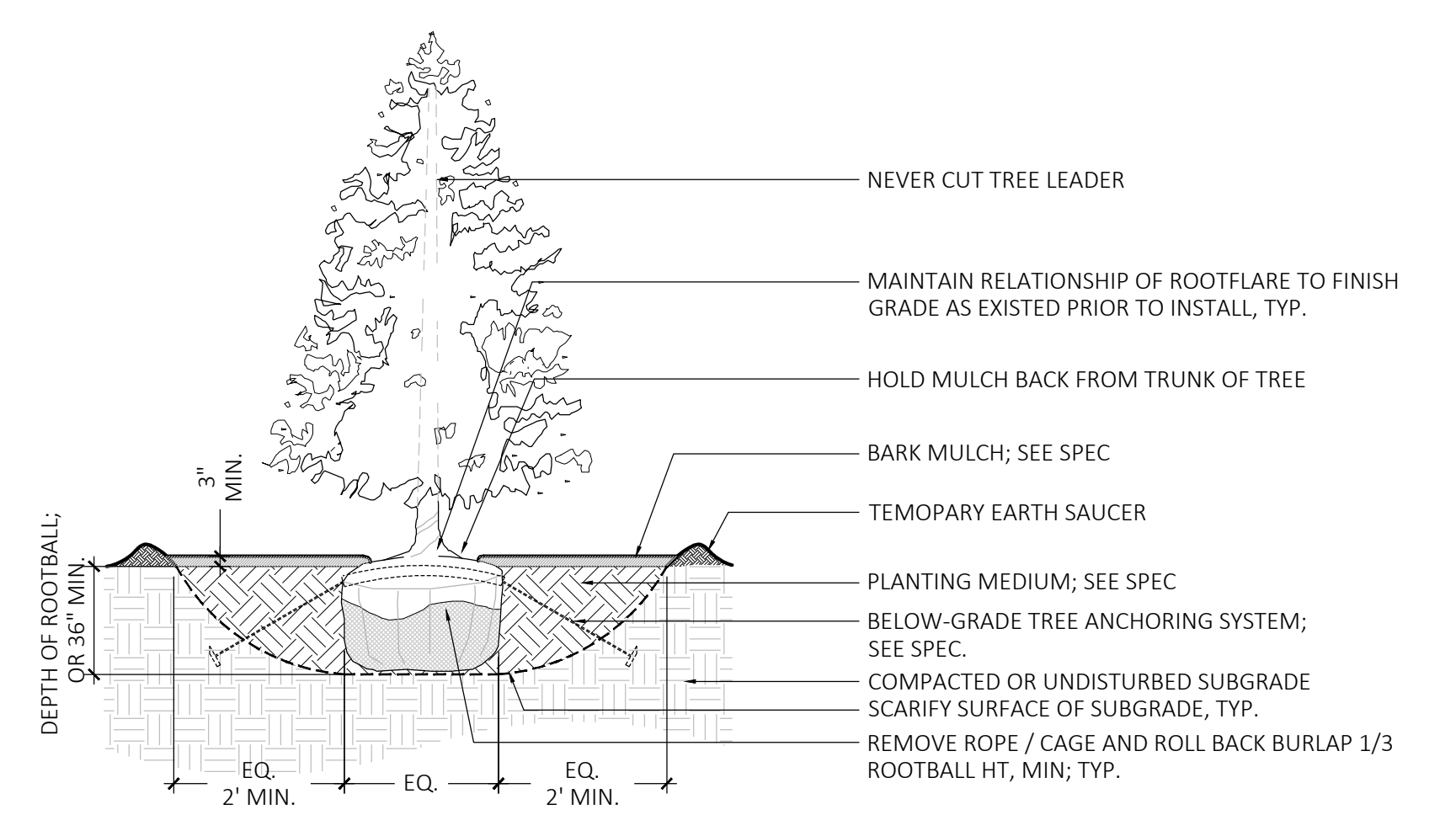
5 EVERGREEN TREE PLANTING SCALE: 3/8" = 1'-0"
