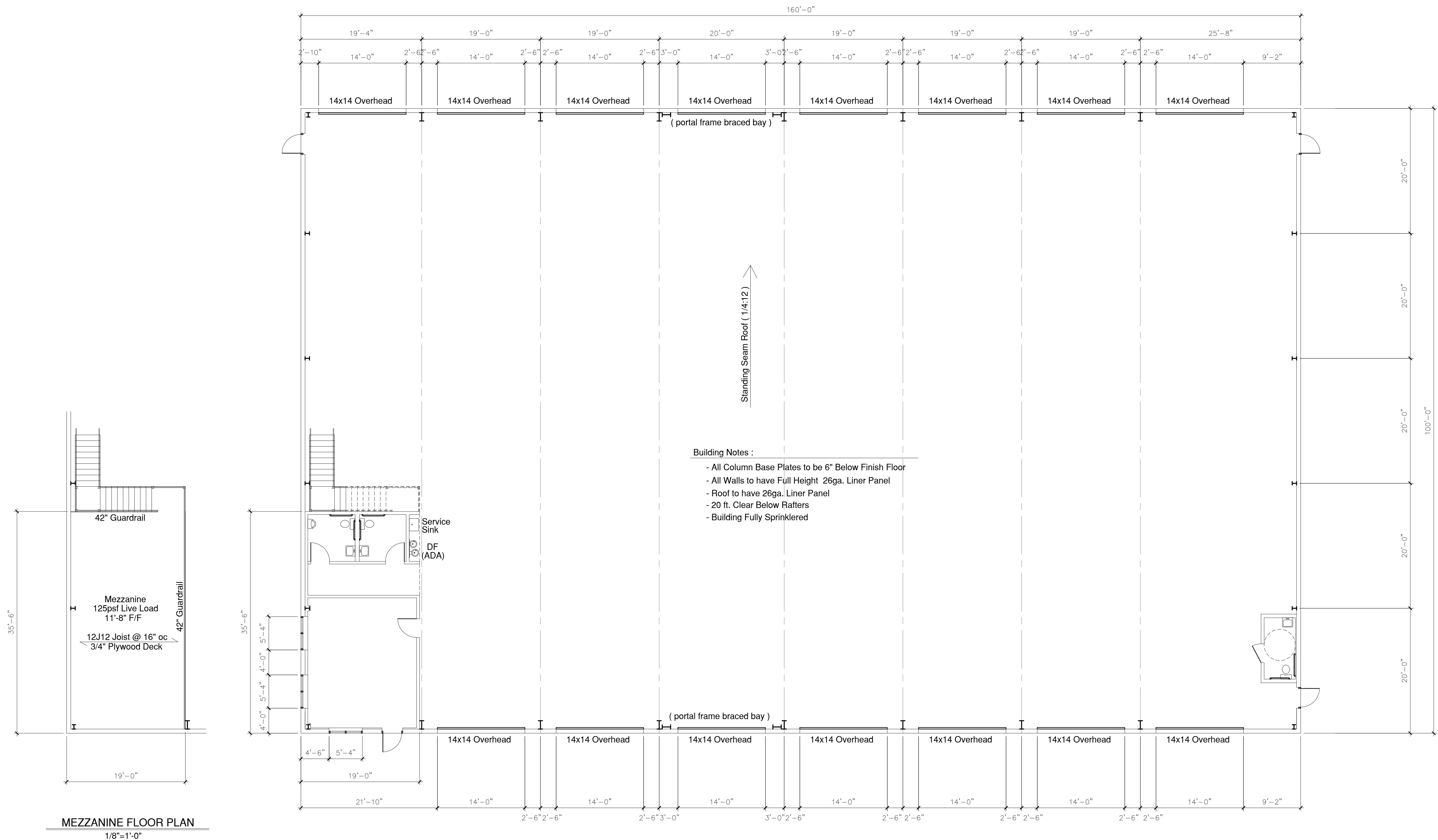
FLOOR PLAN 1/8"=1'-0"
