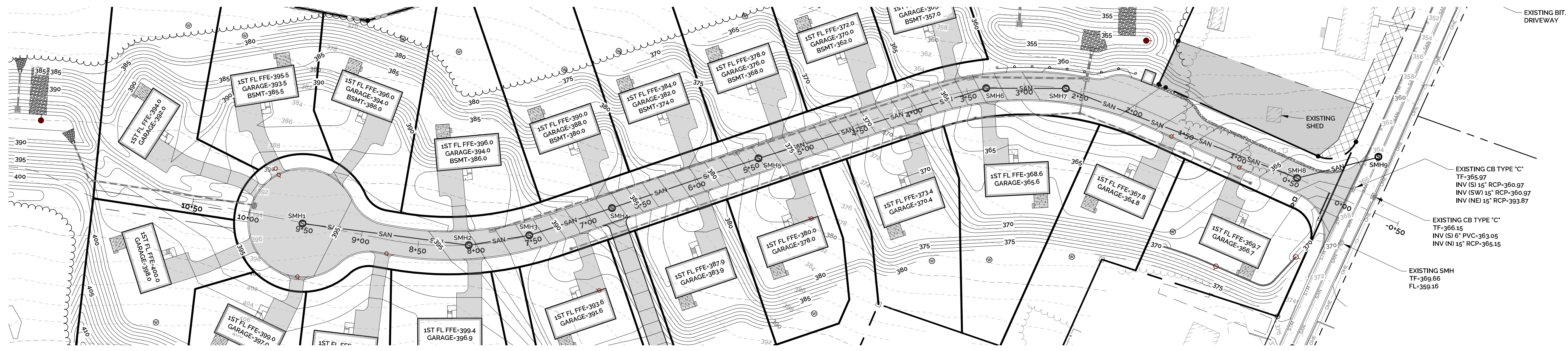
PROPOSED ROADWAY ALIGNMENT SCALE: 1"=50'
