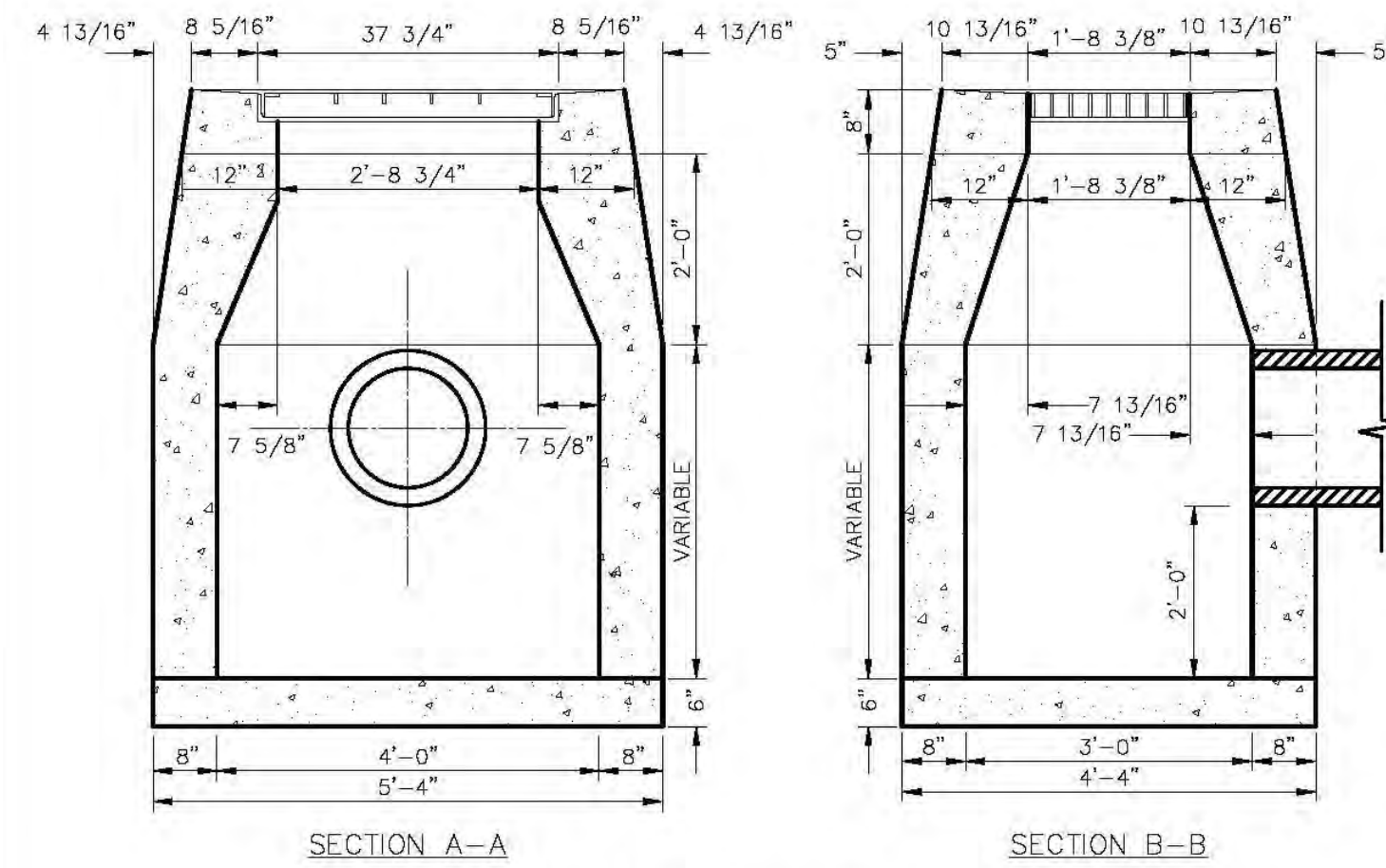
TYPE "C-L" CATCH BASIN DETAIL NOT TO SCALE
