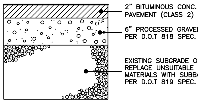
TYPICAL DRIVEWAY SECTION DETAIL NOT TO SCALE
