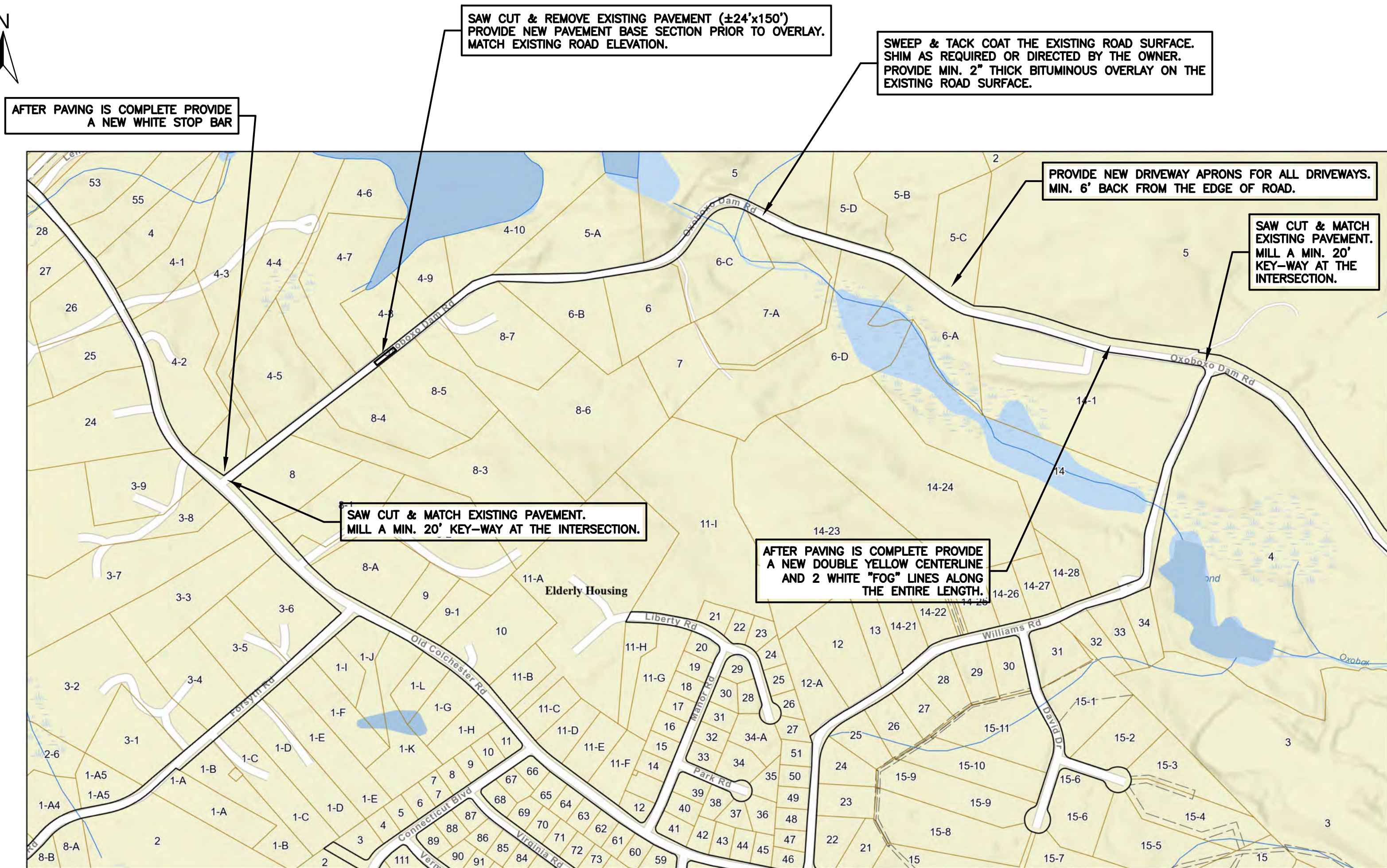
OXOBOXO DAM ROAD PLAN SCALE: 1"=±400'
