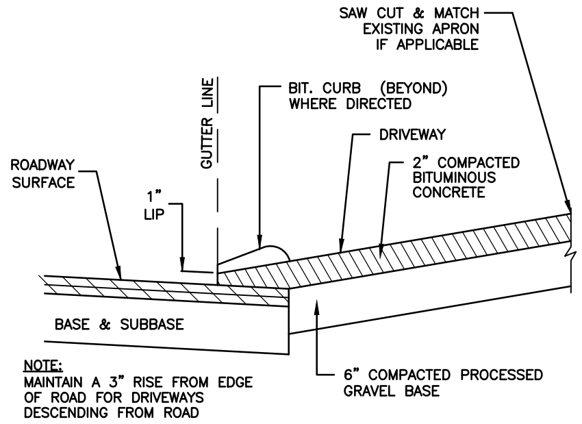
BITUMINOUS CONCRETE DRIVEWAY APRON NOT TO SCALE
