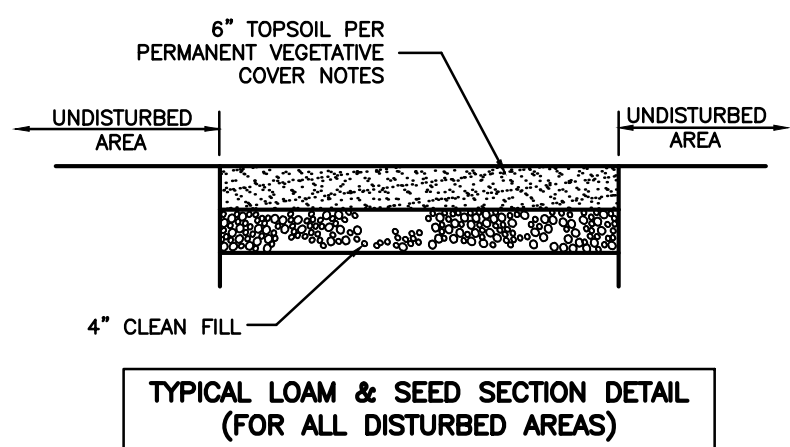
TYPICAL LOAM & SEED SECTION DETAIL (FOR ALL DISTURBED AREAS) NOT TO SCALE
