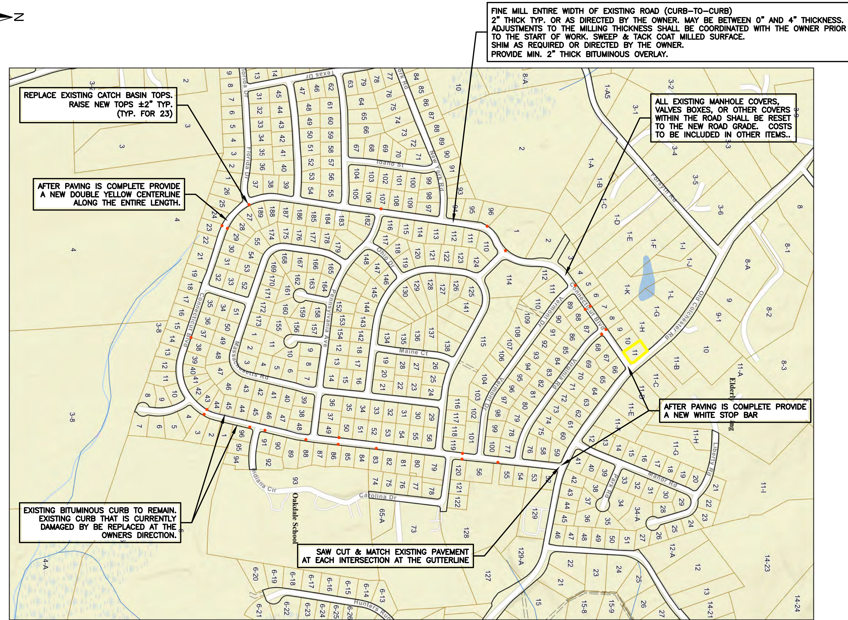
CONNECTICUT BOULEVARD PLAN SCALE: 1"=±400'
