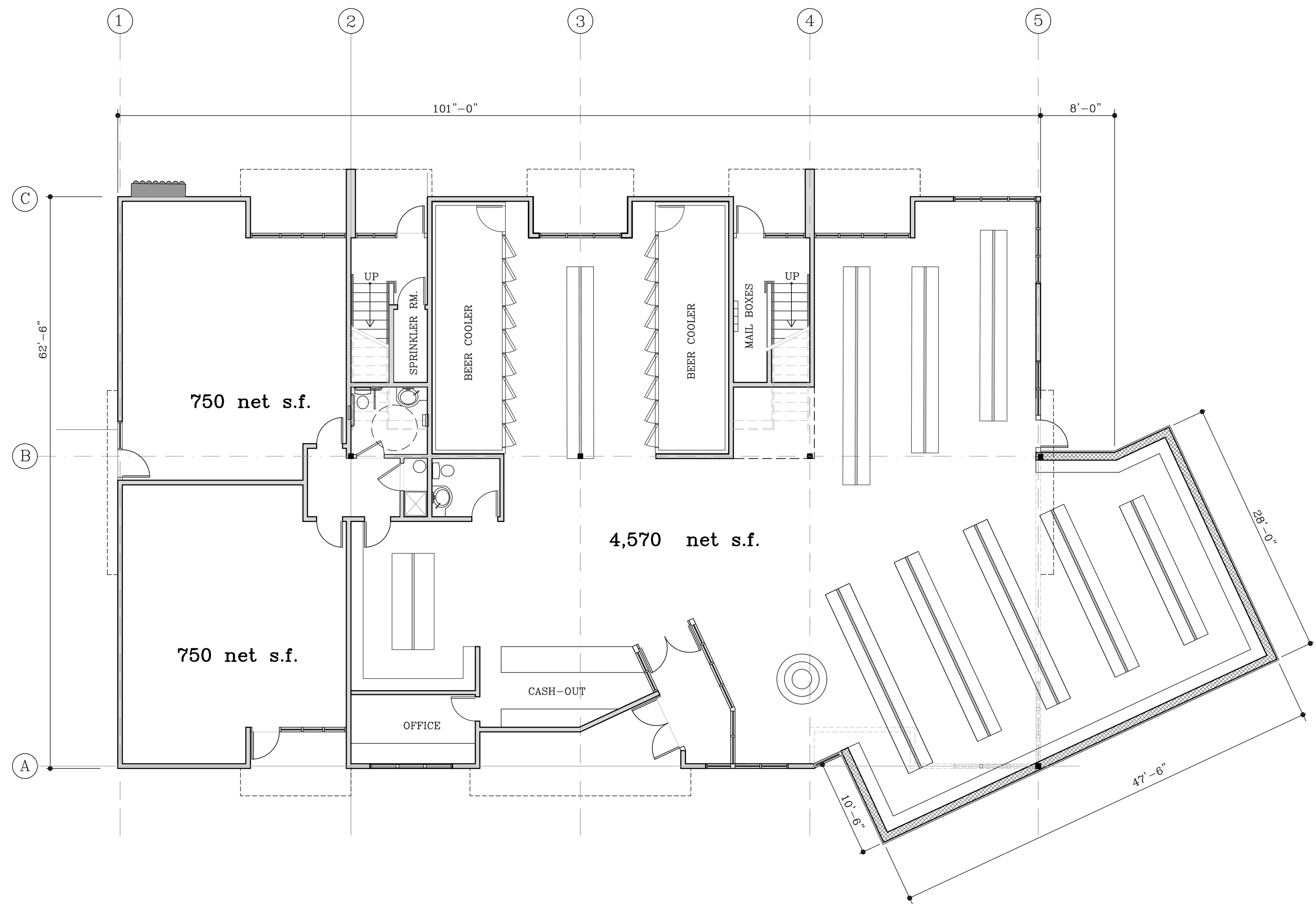
1 FIRST FLOOR PLAN SCALE: 1/8" = 1'0"
