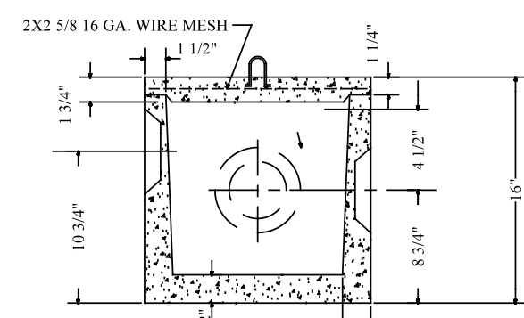
STANDARD D-BOX NOT TO SCALE
