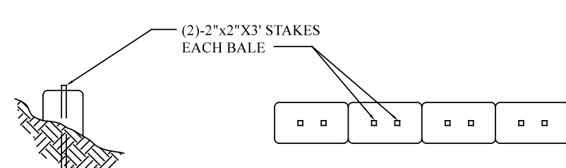
HAYBALE BARRIER NOT TO SCALE
