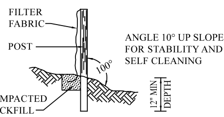
SILT FENCE NOT TO SCALE
